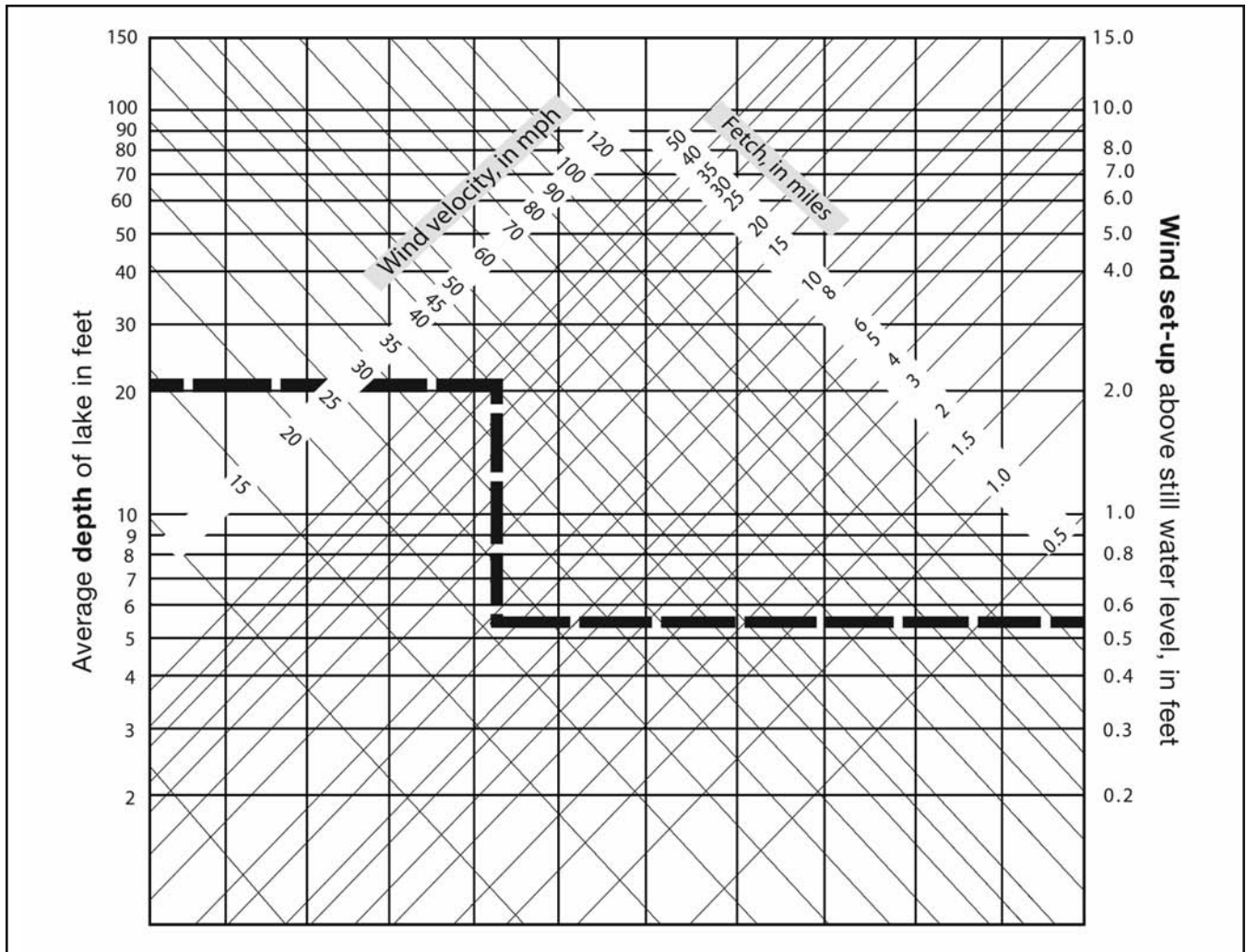
Figure 10: Diagram for determining wind setup on lakes. For example, ( — — — ) a wind of 40 mph blowing across a lake with an average depth of 20 ft. and a fetch of 10 mi. would result in a wind setup of about 0.6 ft.
