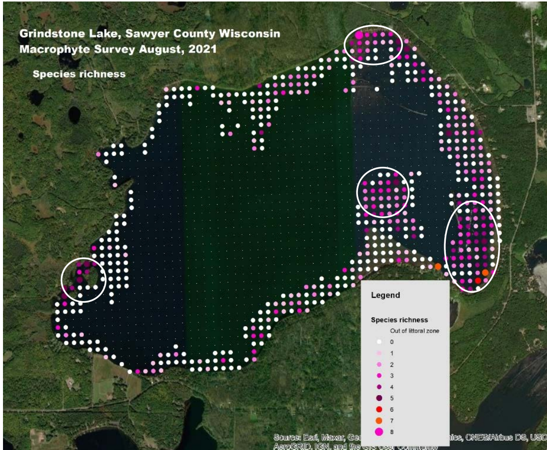
FIGURE 18. SPECIES RICHNESS 2021 AQUATIC PLANT SURVEY
