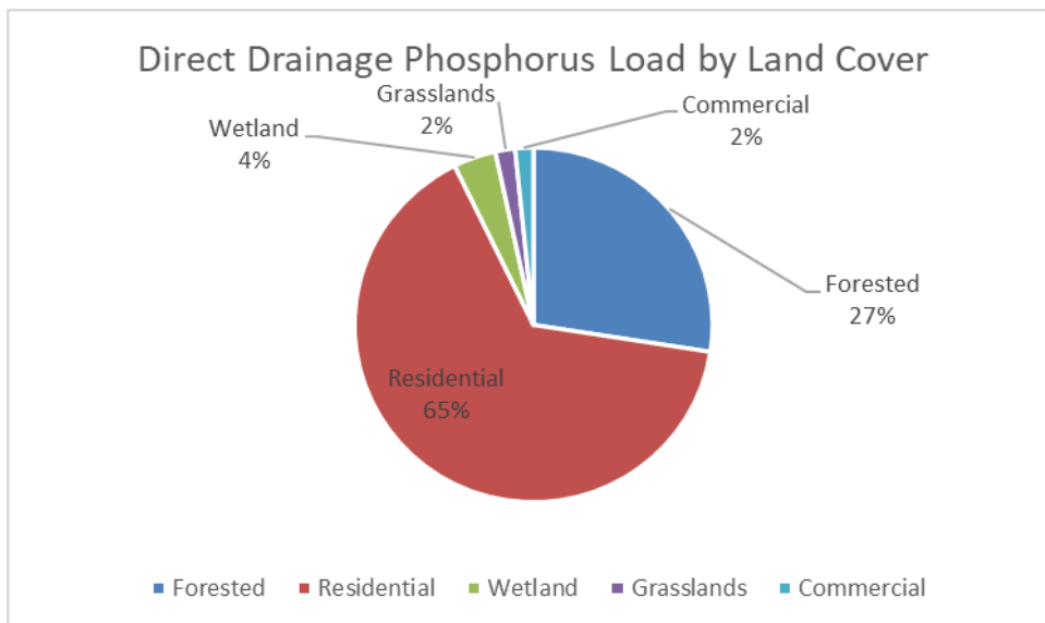
FIGURE 15. PHOSPHORUS LOADING BY LAND COVER DIRECT-DRAINAGE WATERSHED
